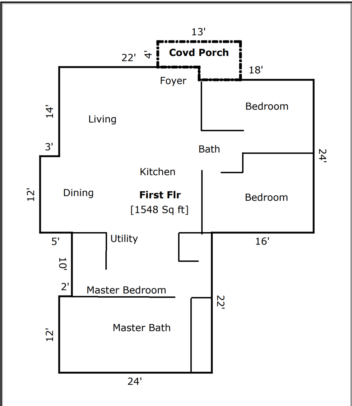
Floor Plan
