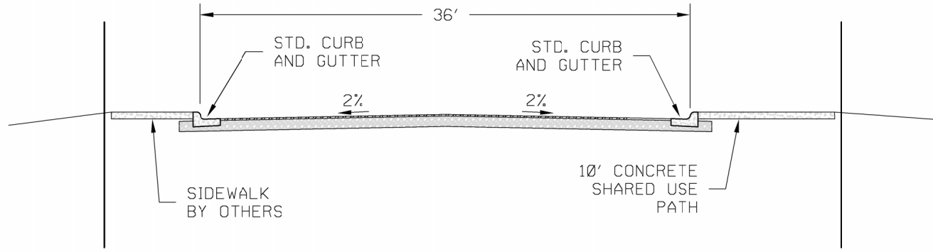
A SAENGERHALLE RD WIDENING STREET SECTION Scale: 1:10
