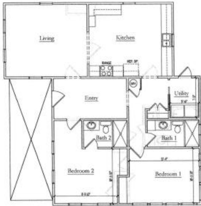
FLOOR PLAN 1
