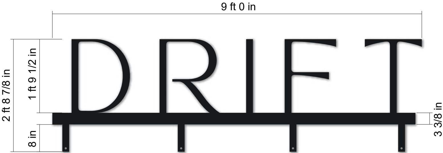
ST.1 WATERJET-CUT LETTERS SCALE: 3/4" = 1'
