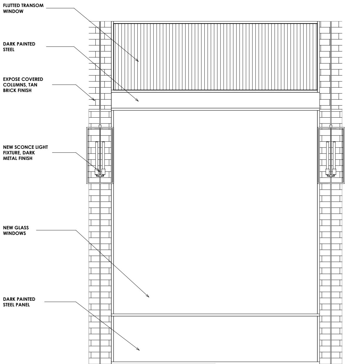
Proposed Elevation
