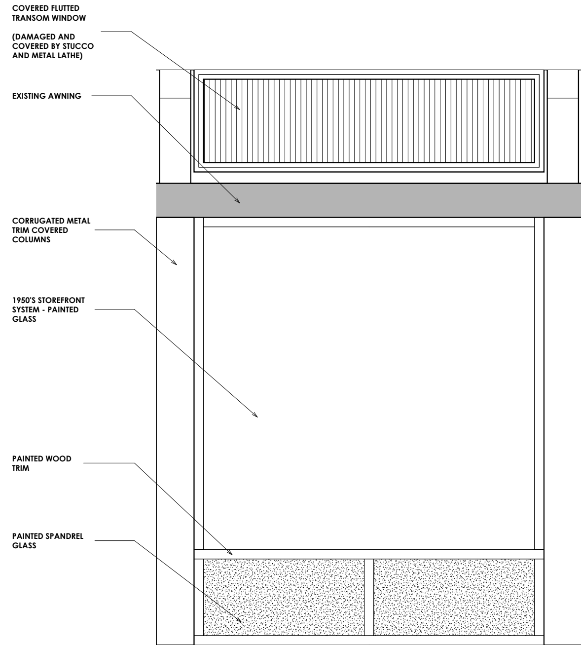
Existing Elevation
