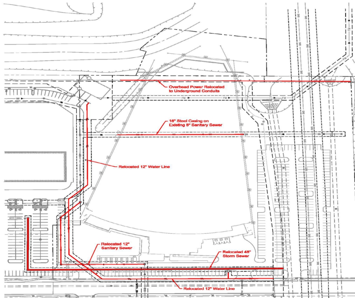
TOP GOLF AT CREEKSIDE TOWN CENTER UTILITY RELOCATIONS
