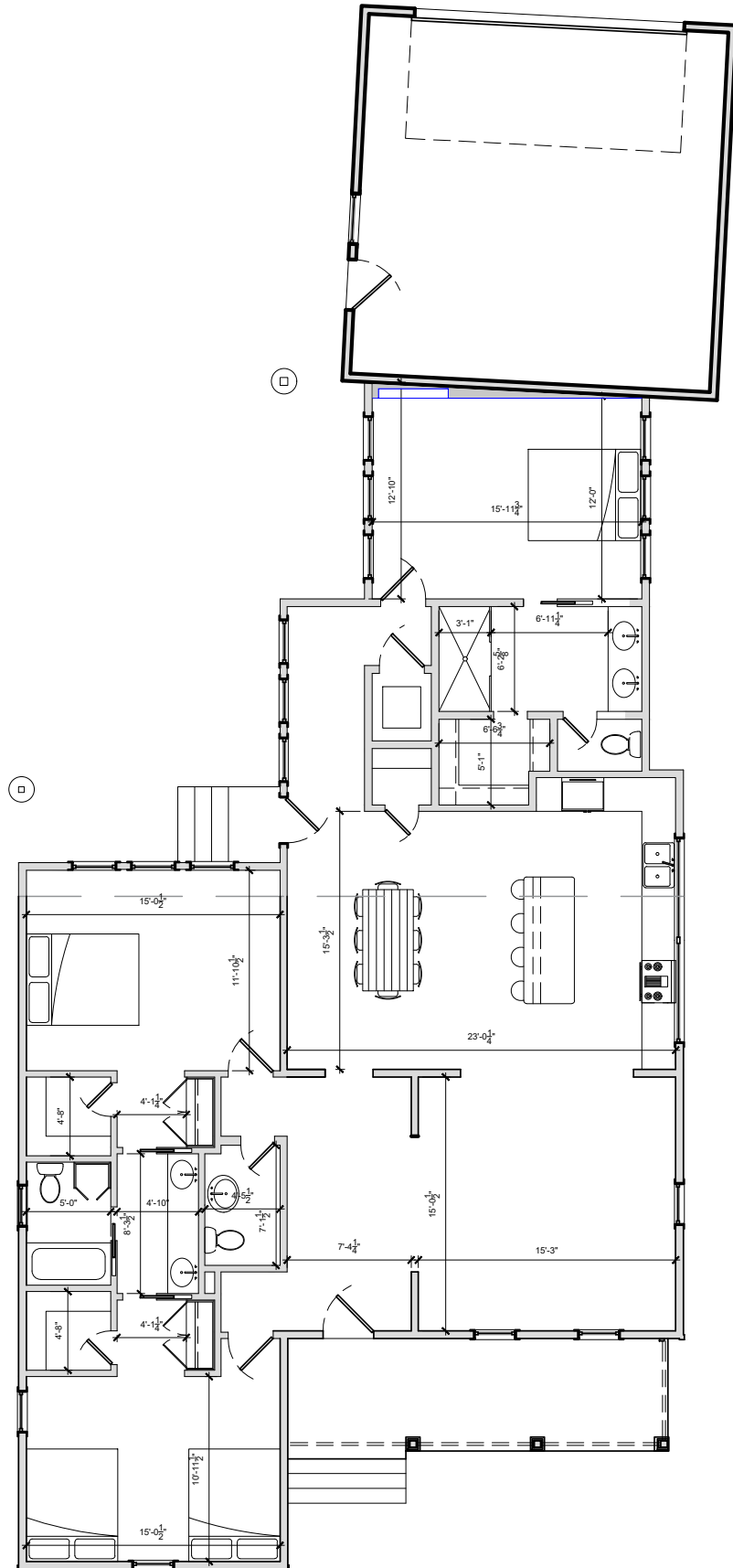
FLOORPLAN
