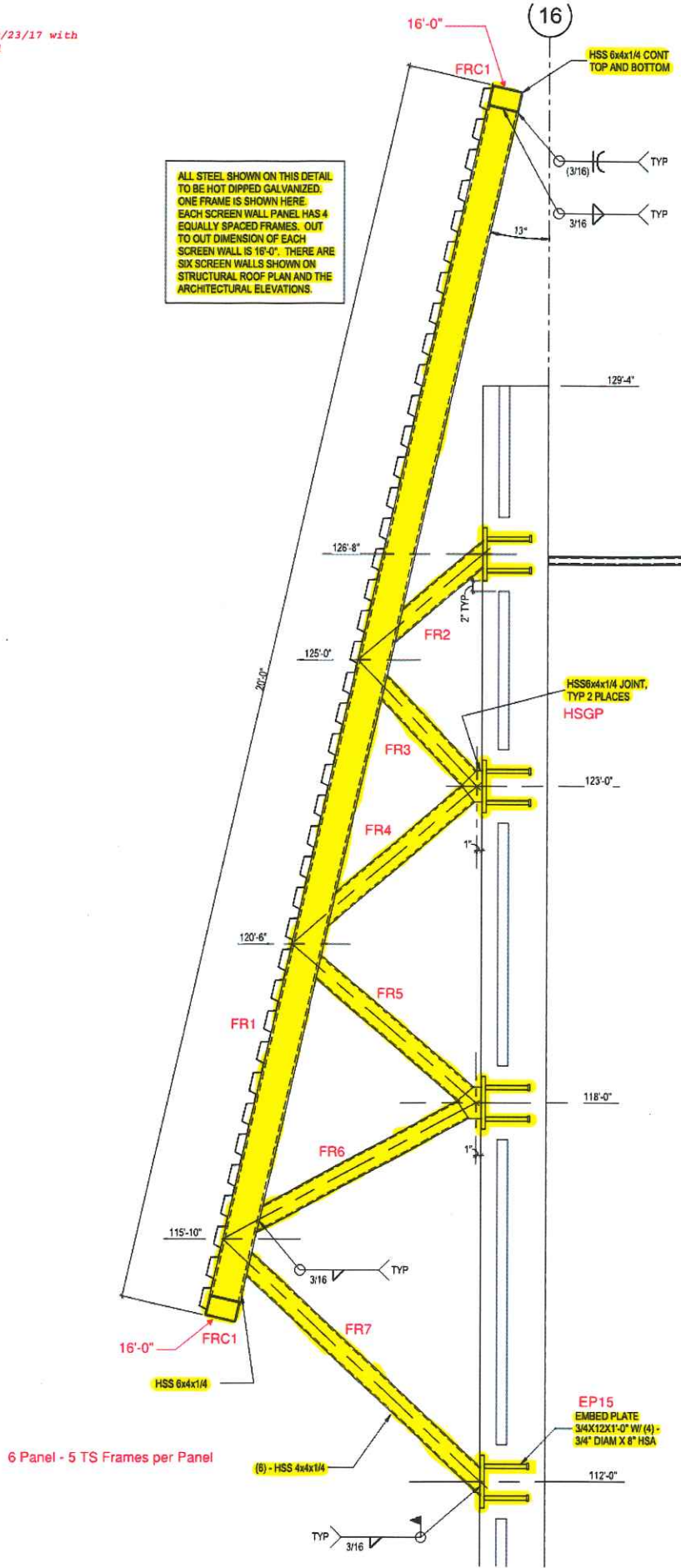
4 Exterior Screen Wall 3/4" = 1'-0"
