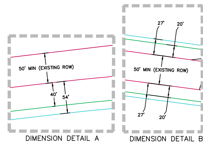
DIMENSION DETAIL A
