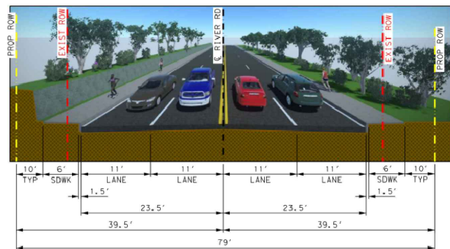
TYPICAL ROADWAY SECTION
