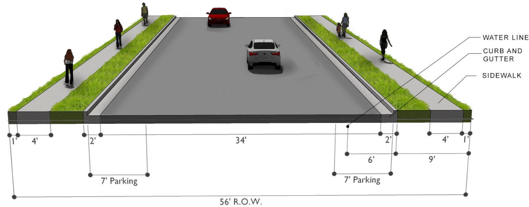
Figure 8-2 Cross Sections – Local B Street
