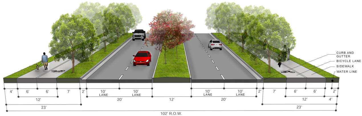
Figure 8-6 Cross Sections – Major Collector w/ Bicycle Lane
