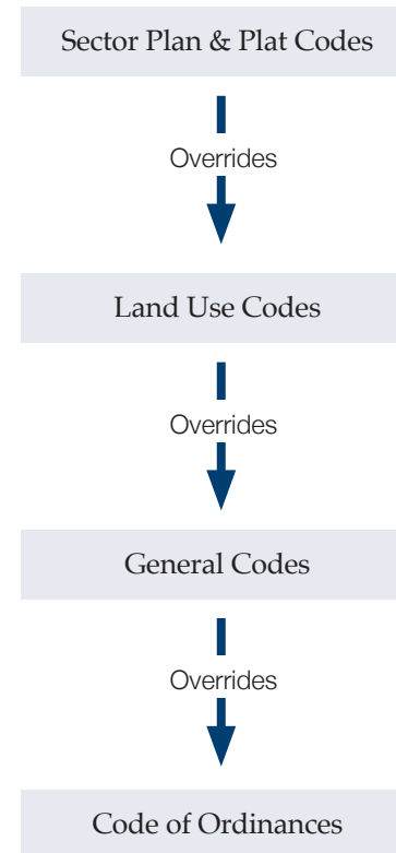
Figure 2-2 Code Hierarchy
