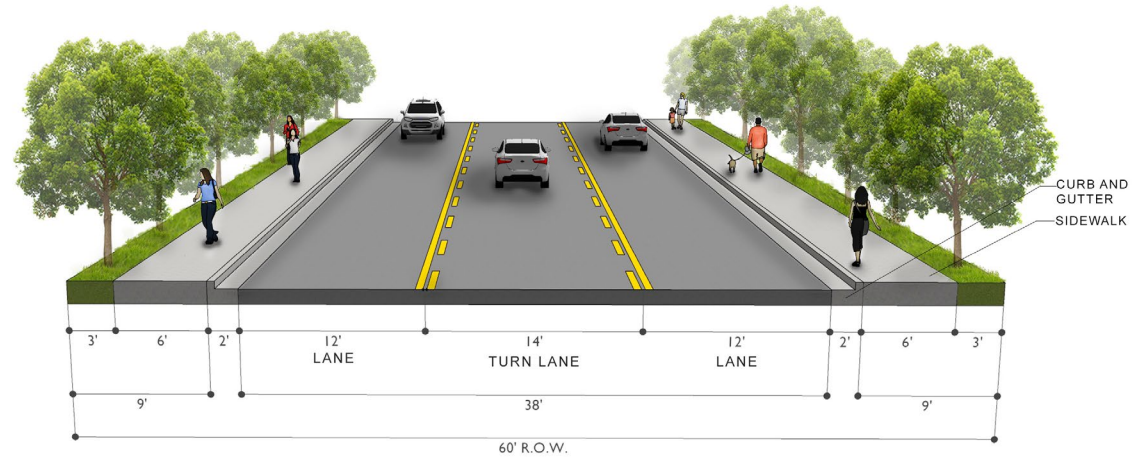
Figure 8-3 Cross Sections – Minor Collector
