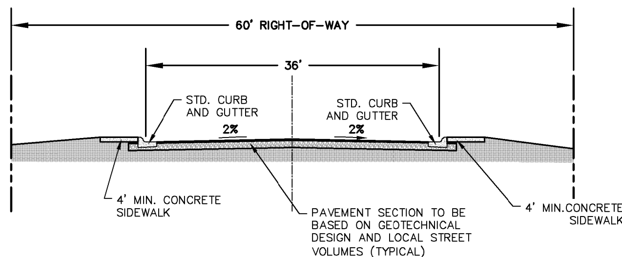
B 36' STANDARD STREET SECTION
