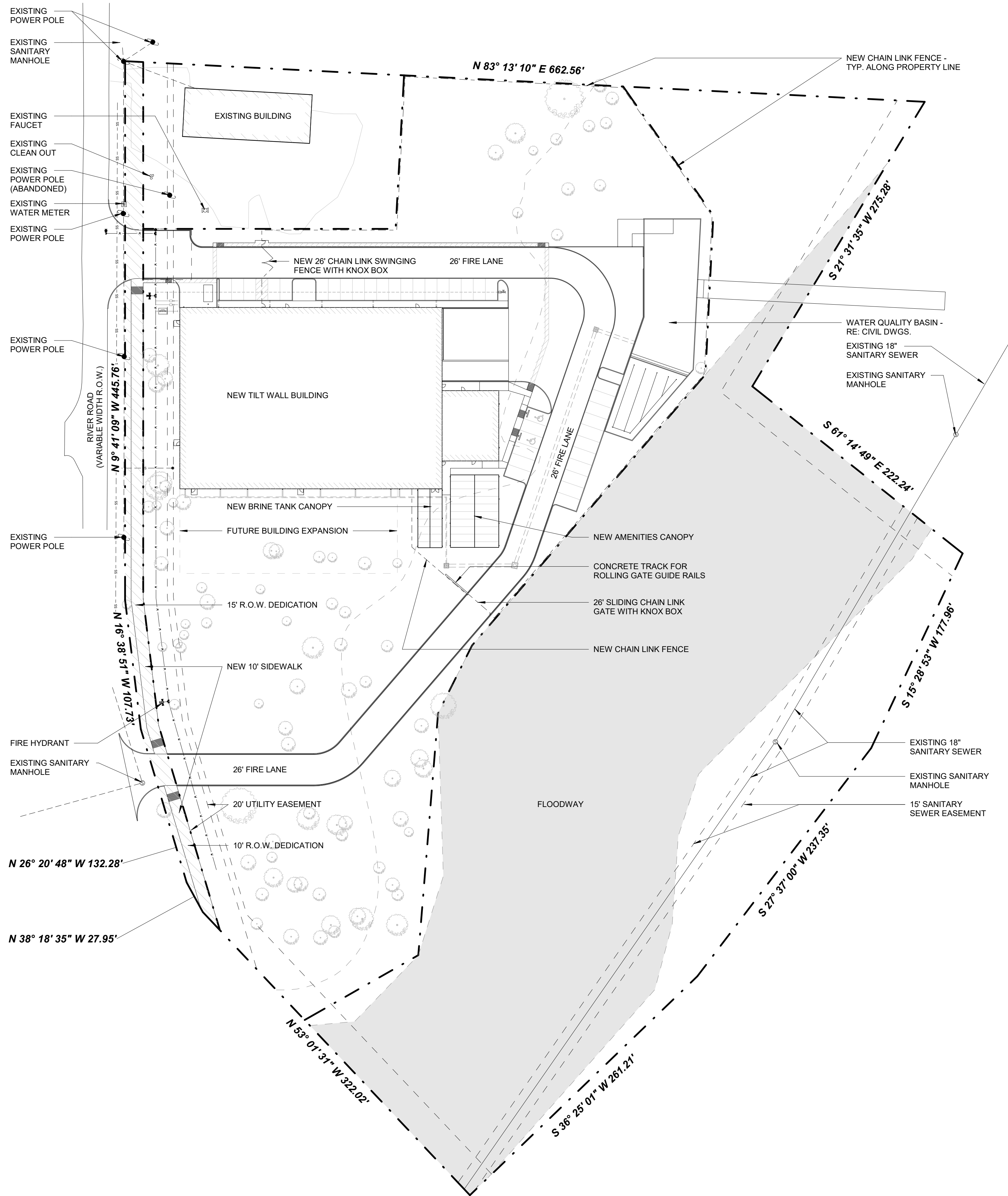
1 OVERALL SITE PLAN A0.4 1" = 50'-0"
