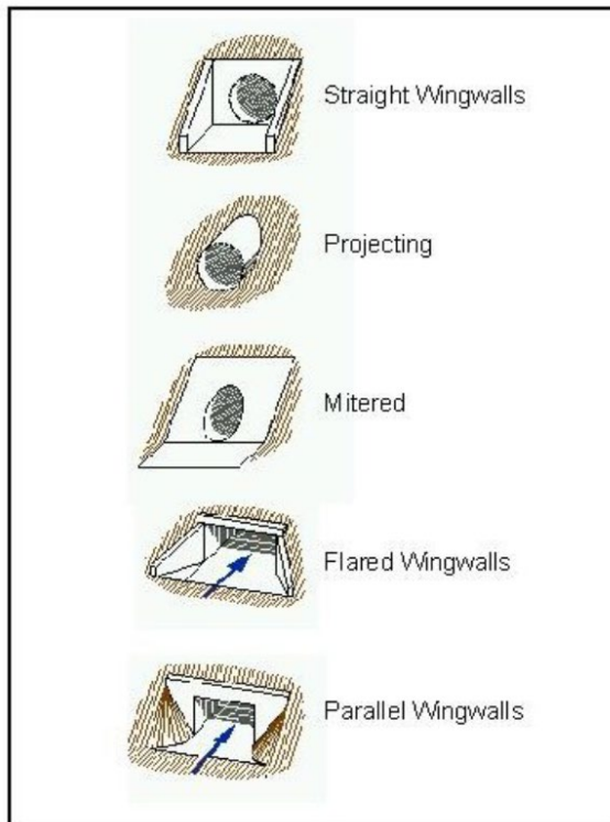
Figure 9-1: Typical Culvert End Treatments
